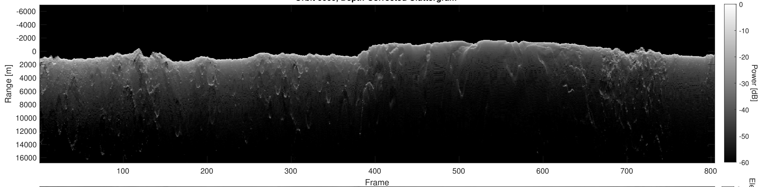
Orbit 6660, Depth-Corrected Cluttergram
