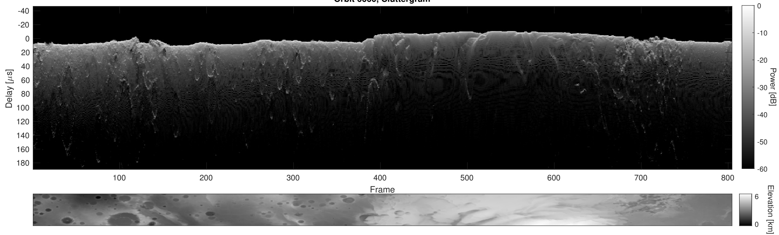
Orbit 6660, Cluttergram
