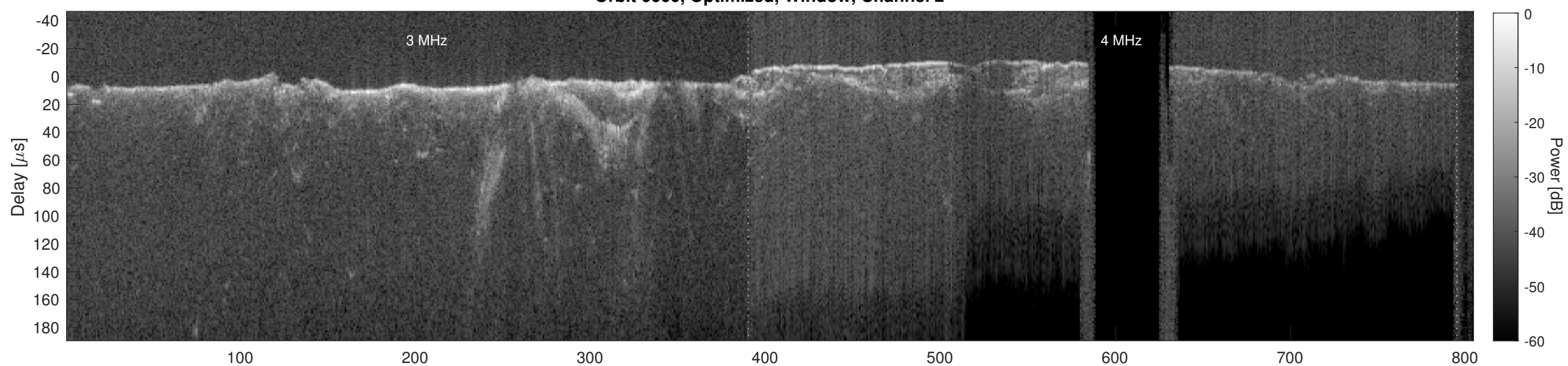
Orbit 6660, Cluttergram
