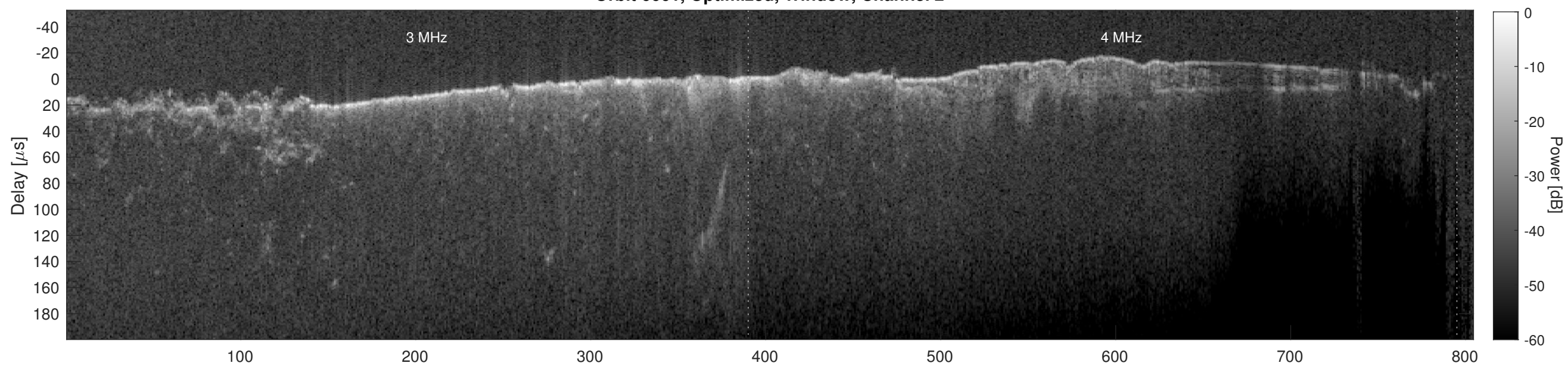
Orbit 6661, Cluttergram
