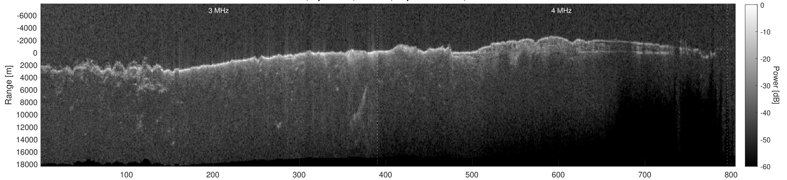
Orbit 6661, Depth-Corrected Cluttergram
