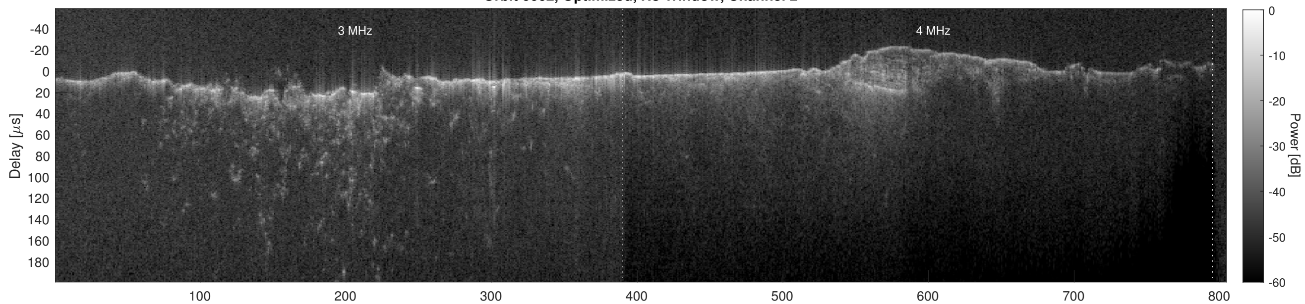
Orbit 6662, Cluttergram
