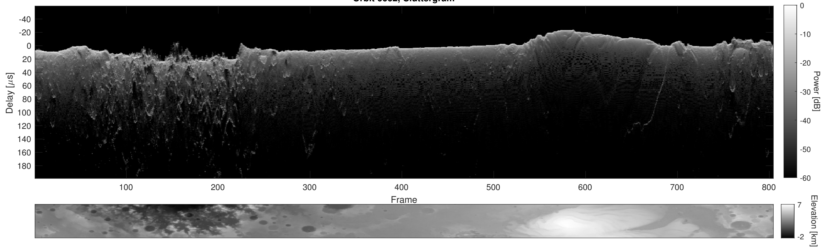
Orbit 6662, Cluttergram
