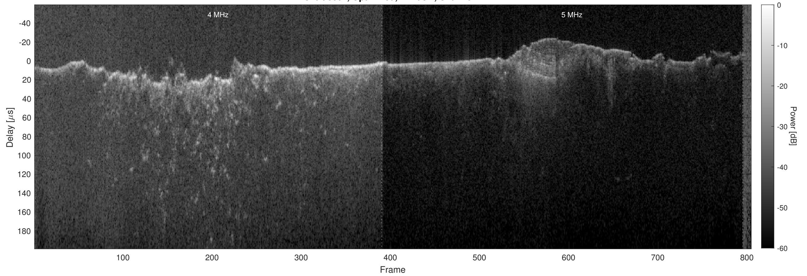
Orbit 6662, Optimized, Window, Channel 2
