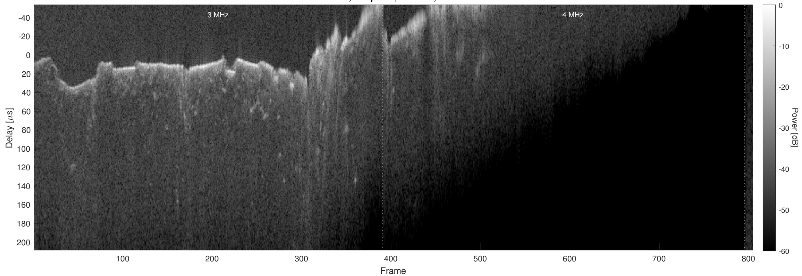
Orbit 6663, Chapman, Window, Channel 2
