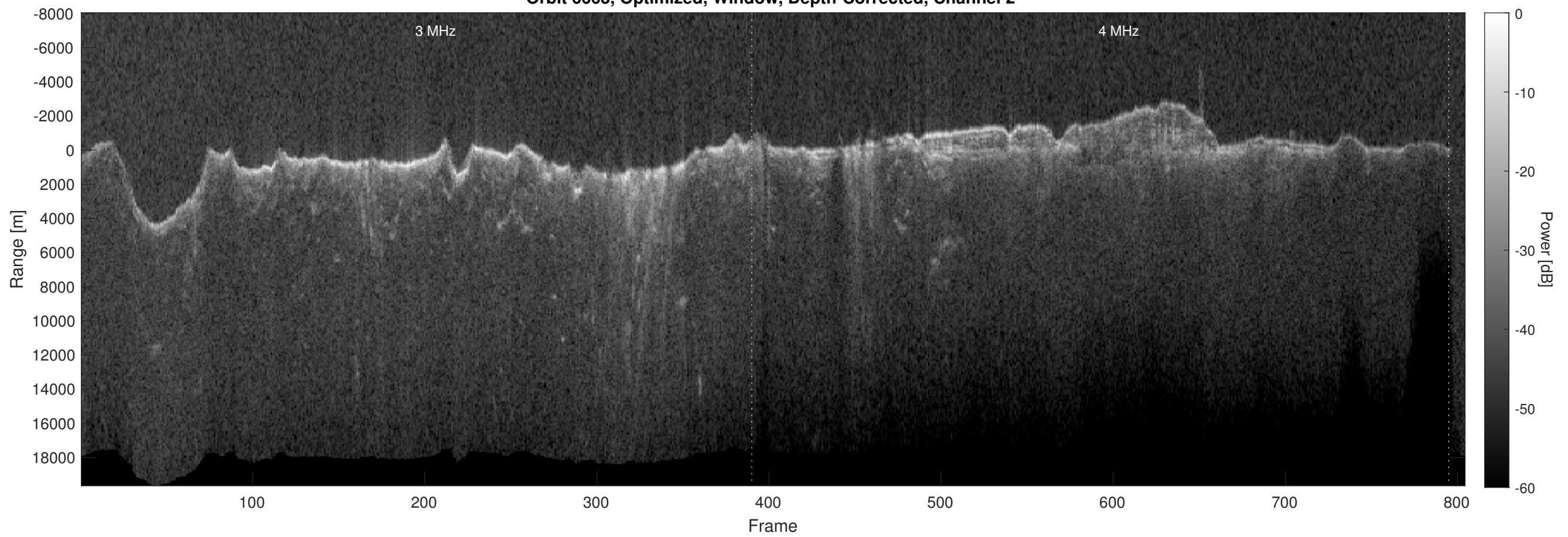
Orbit 6663, Optimized, Window, Depth-Corrected, Channel 2
