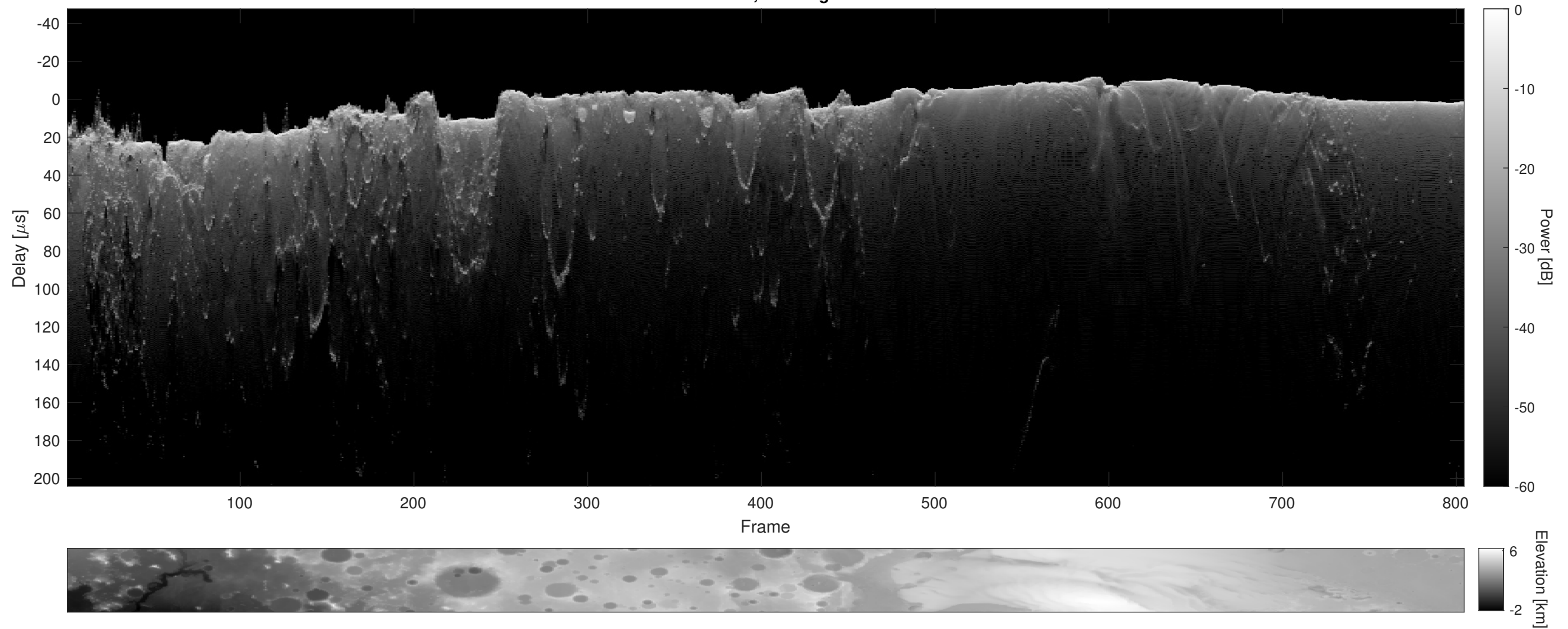
Orbit 6664, Cluttergram
