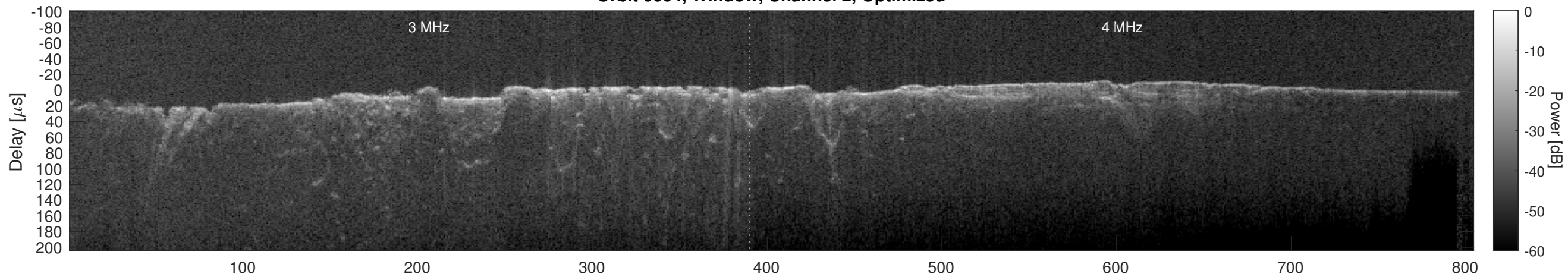
Orbit 6664, Cluttergram
