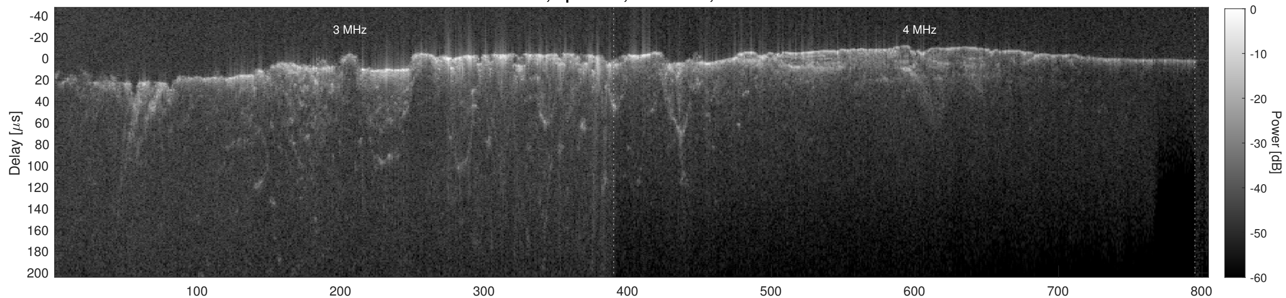
Orbit 6664, Cluttergram
