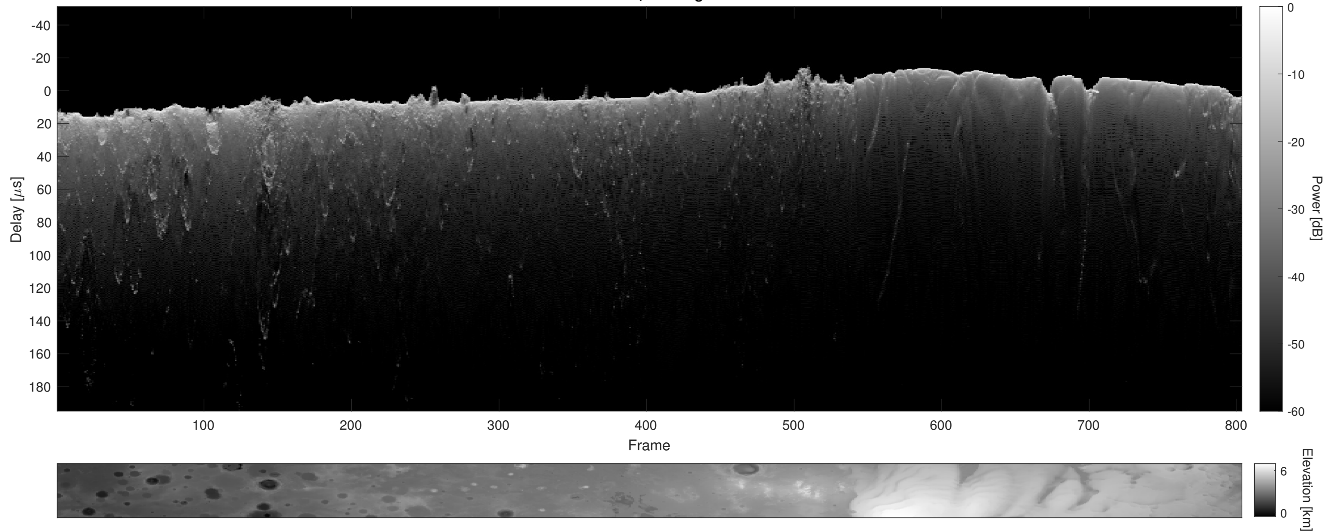
Orbit 6665, Cluttergram
