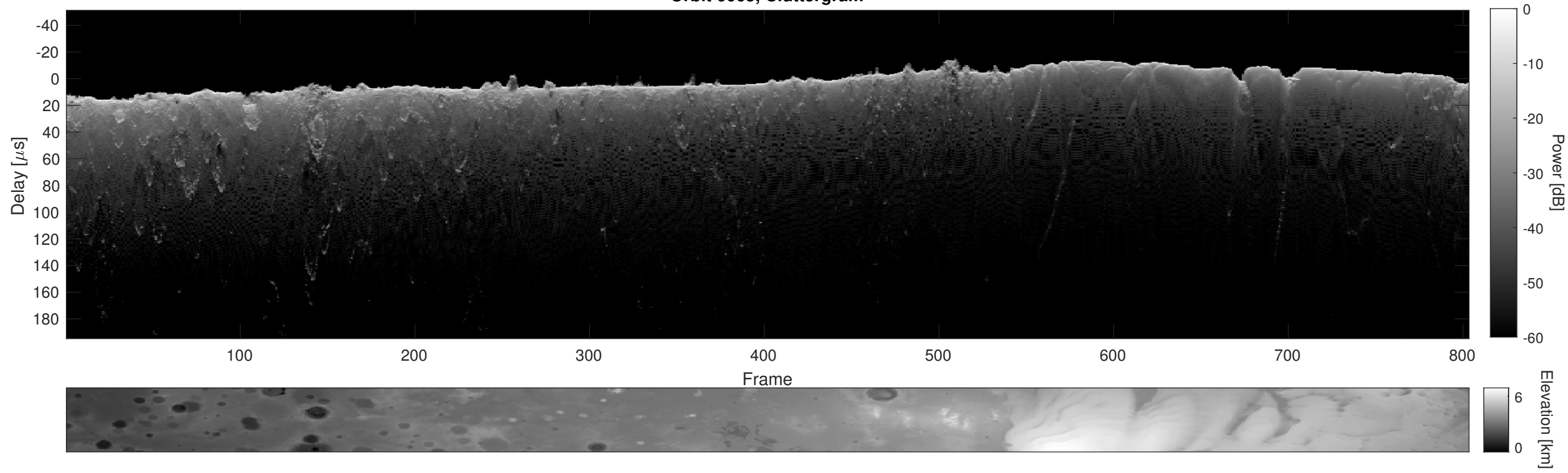
Orbit 6665, Cluttergram
