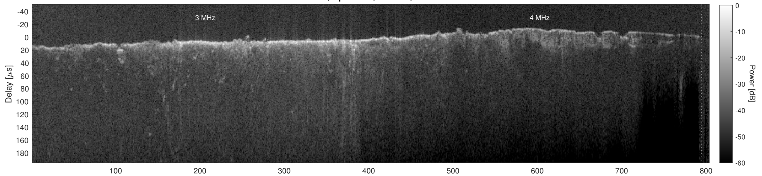
Orbit 6665, Cluttergram
