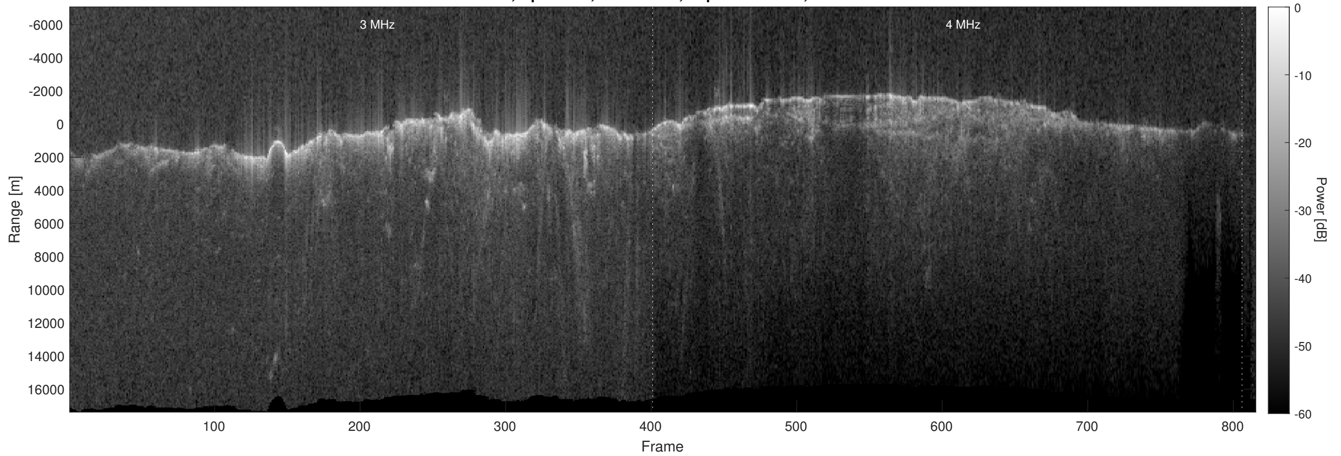
Orbit 6667, Optimized, No Window, Depth-Corrected, Channel 2
