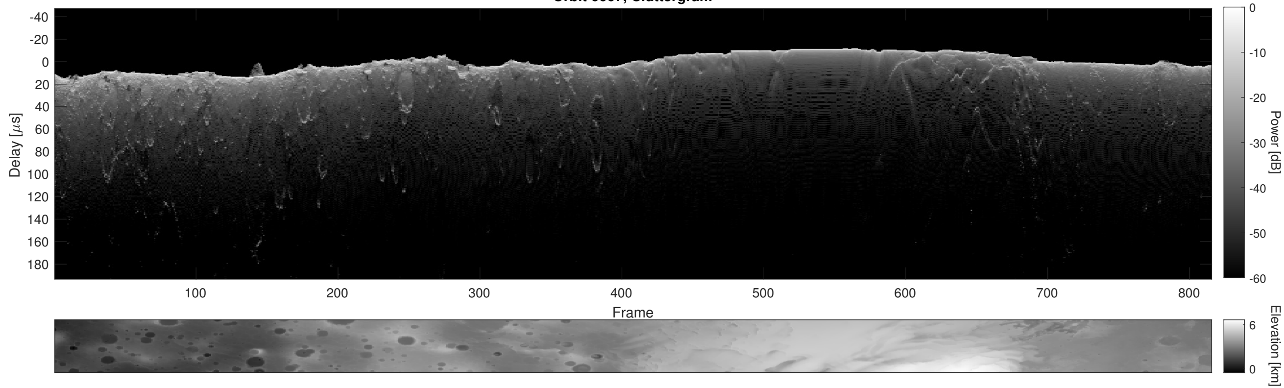
Orbit 6667, Cluttergram
