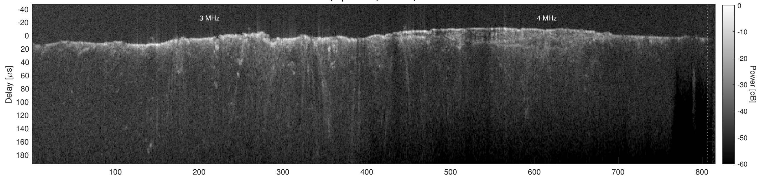
Orbit 6667, Cluttergram
