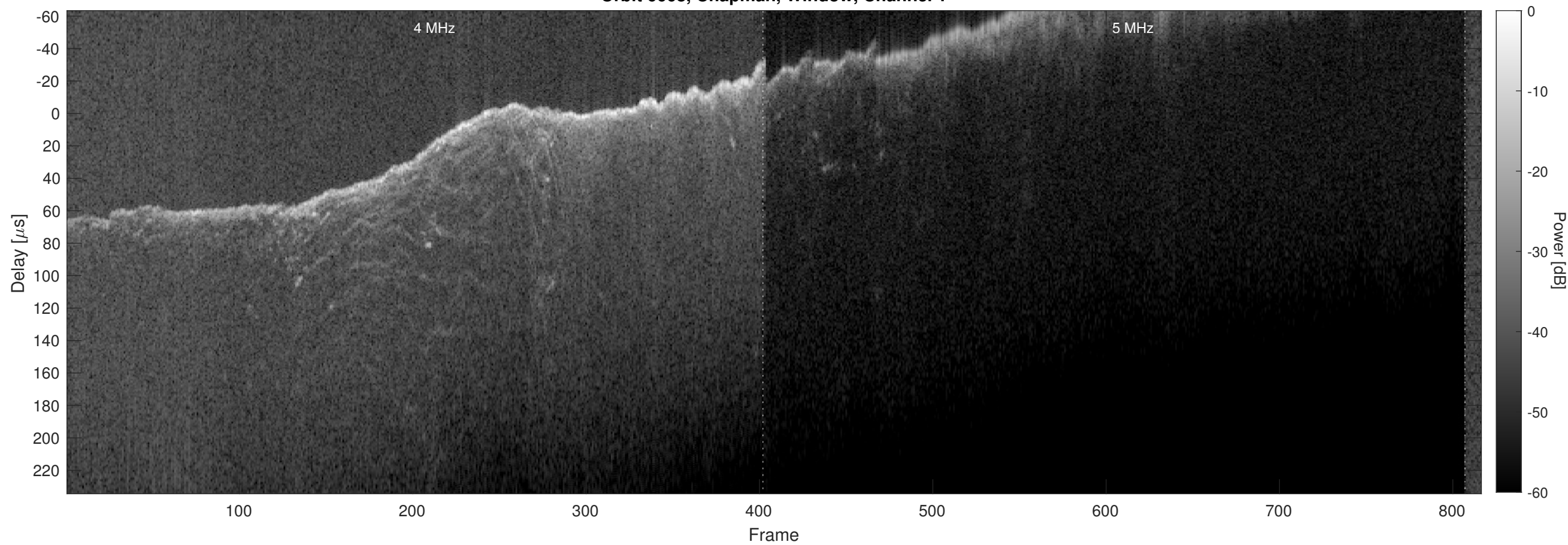
Orbit 6668, Chapman, Window, Channel 2
