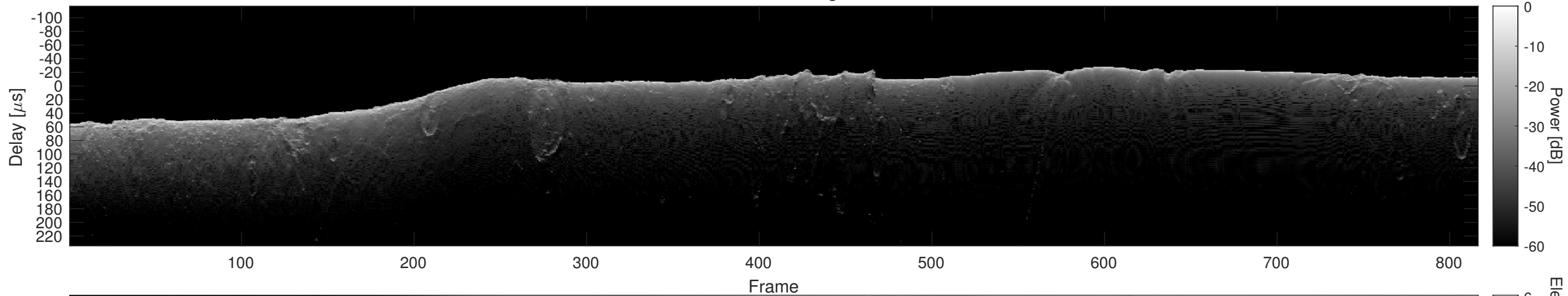
Orbit 6668, Cluttergram
