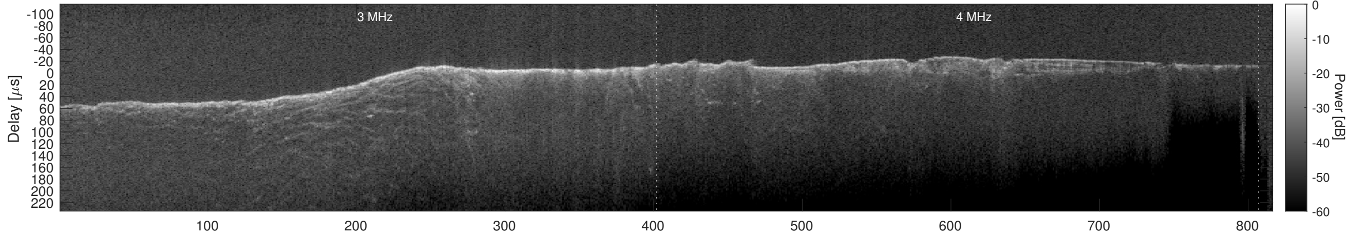
Orbit 6668, Cluttergram
