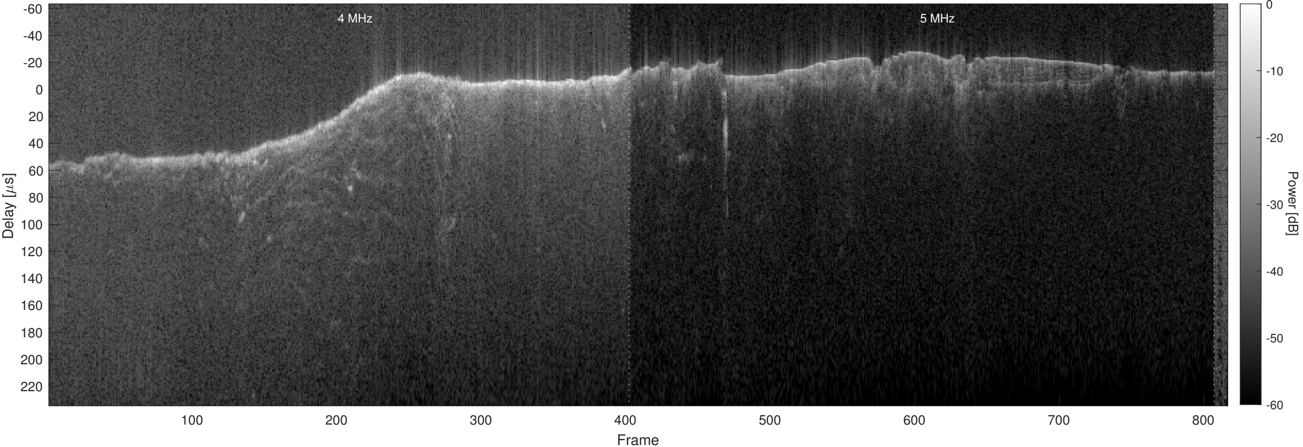
Orbit 6668, Optimized, No Window, Channel 2
