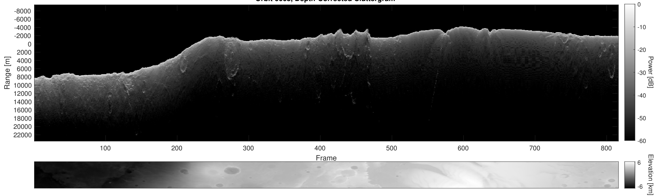
Orbit 6668, Depth-Corrected Cluttergram
