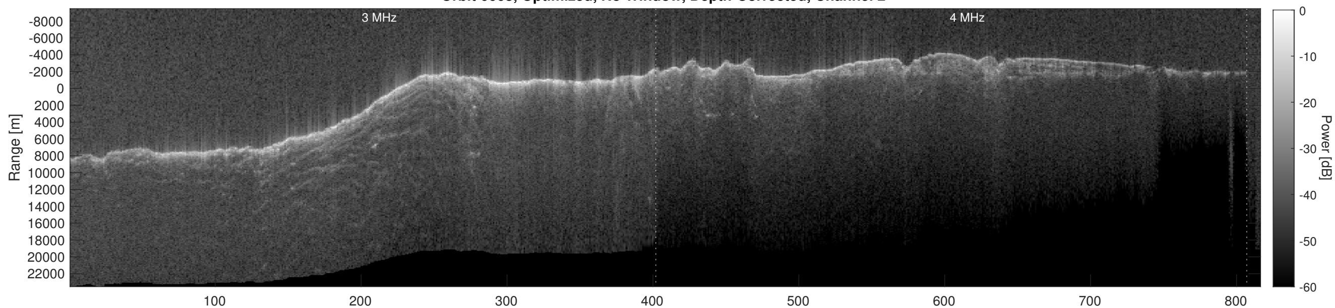
Orbit 6668, Depth-Corrected Cluttergram
