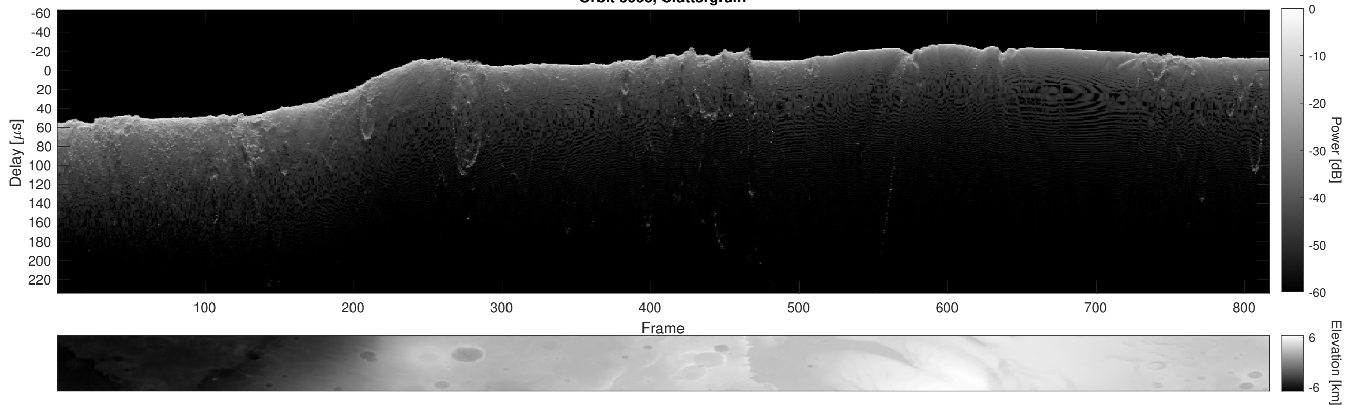
Orbit 6668, Cluttergram
