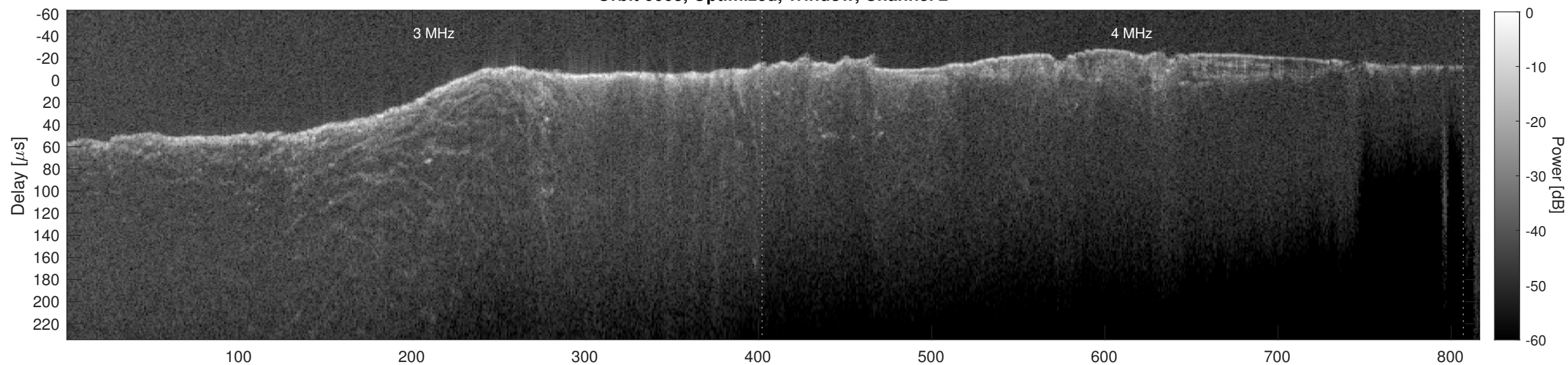
Orbit 6668, Cluttergram
