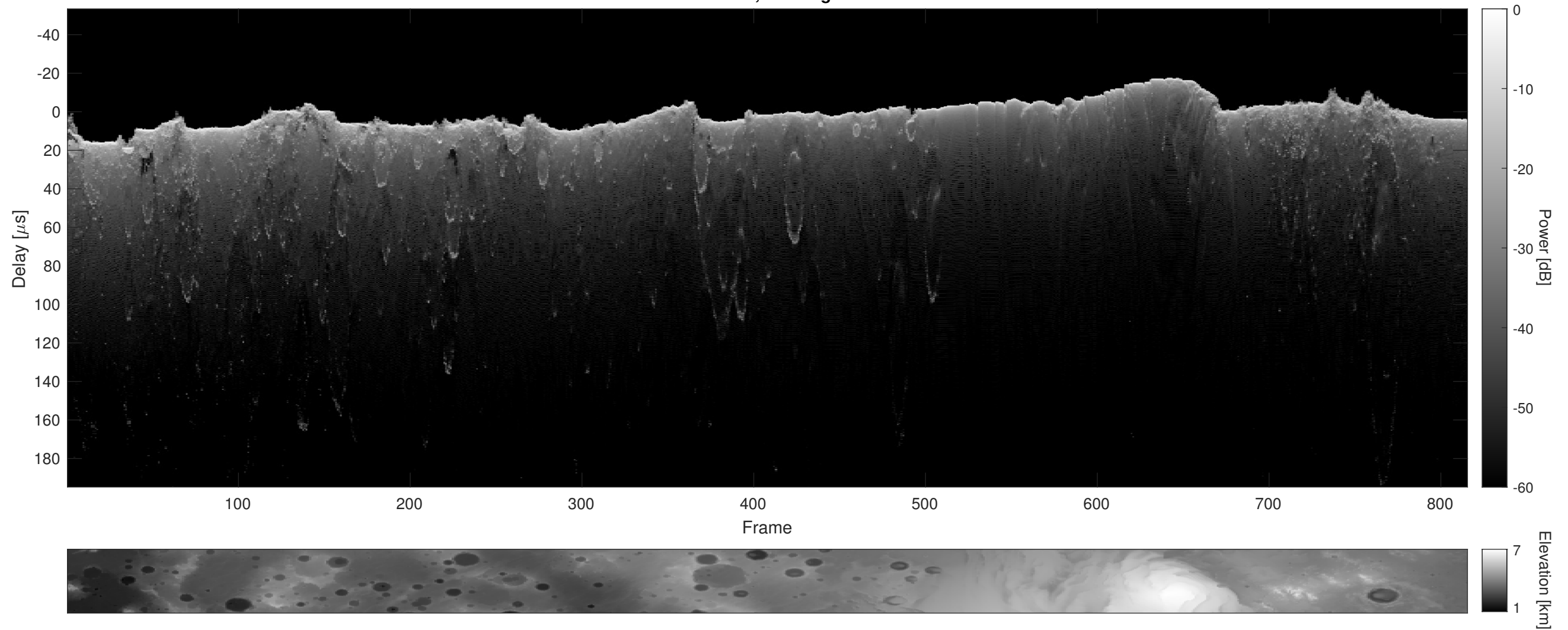
Orbit 6670, Cluttergram
