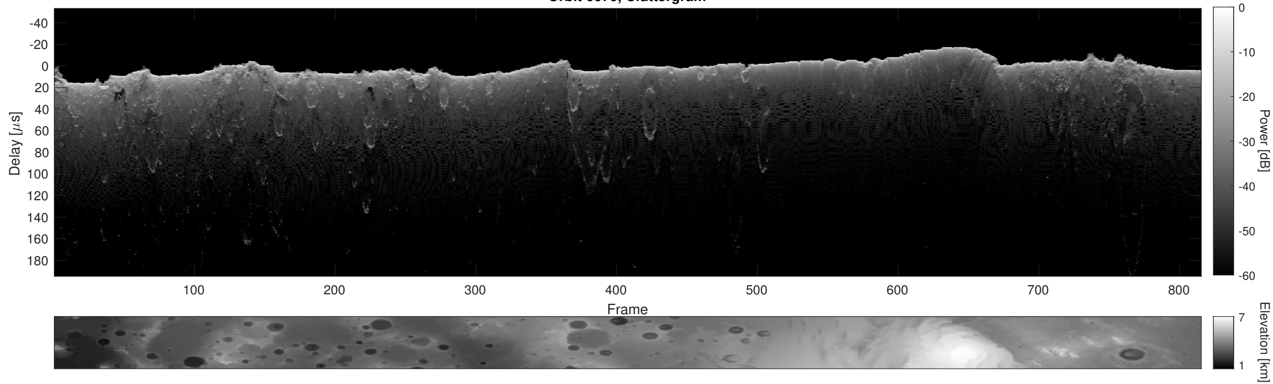
Orbit 6670, Cluttergram
