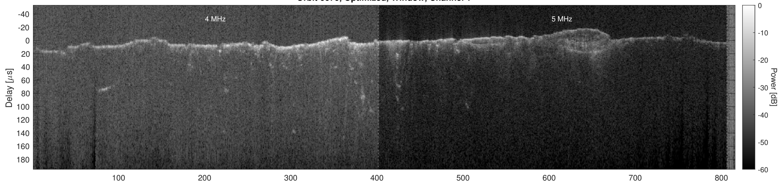
Orbit 6670, Optimized, Window, Channel 2
