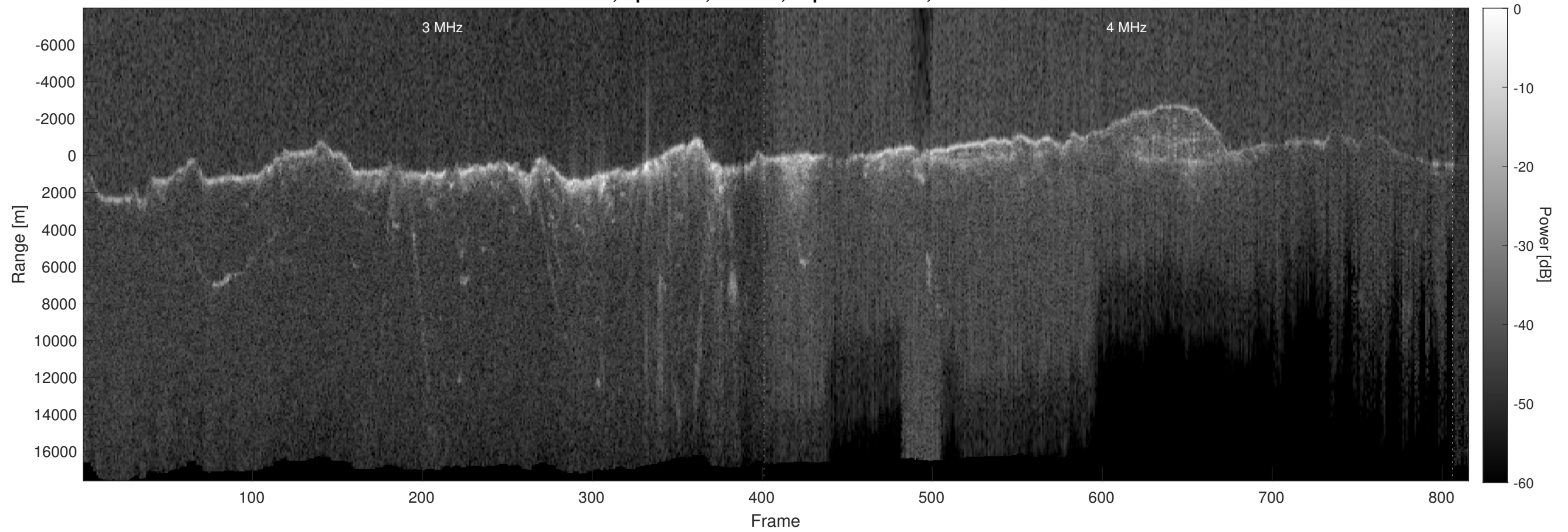
Orbit 6670, Optimized, Window, Depth-Corrected, Channel 2
