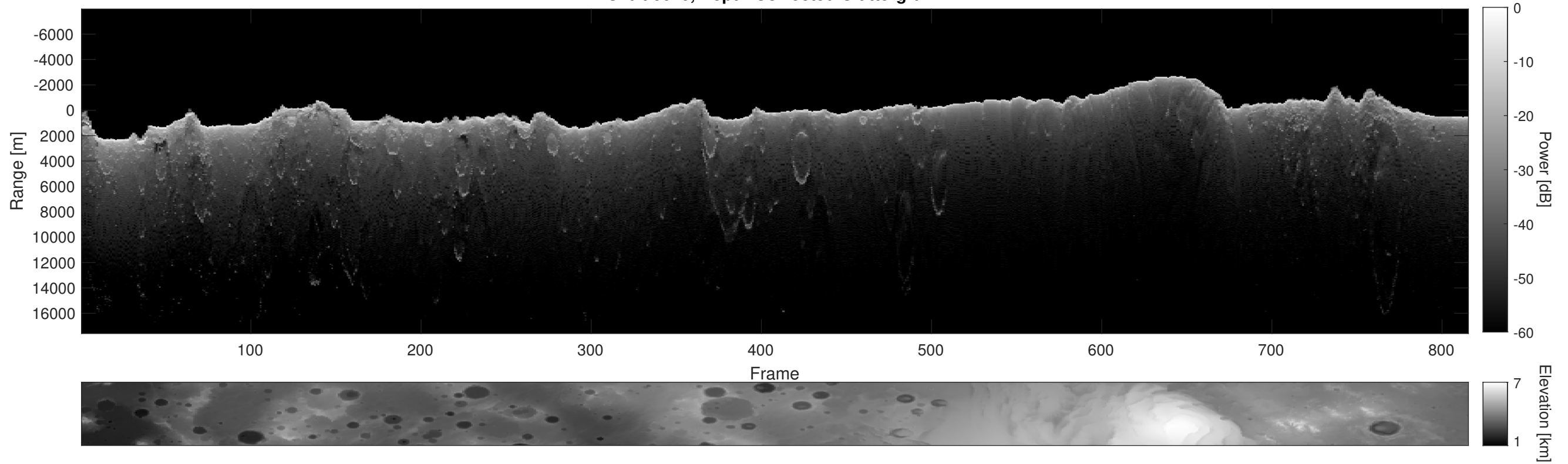
Orbit 6670, Depth-Corrected Cluttergram
