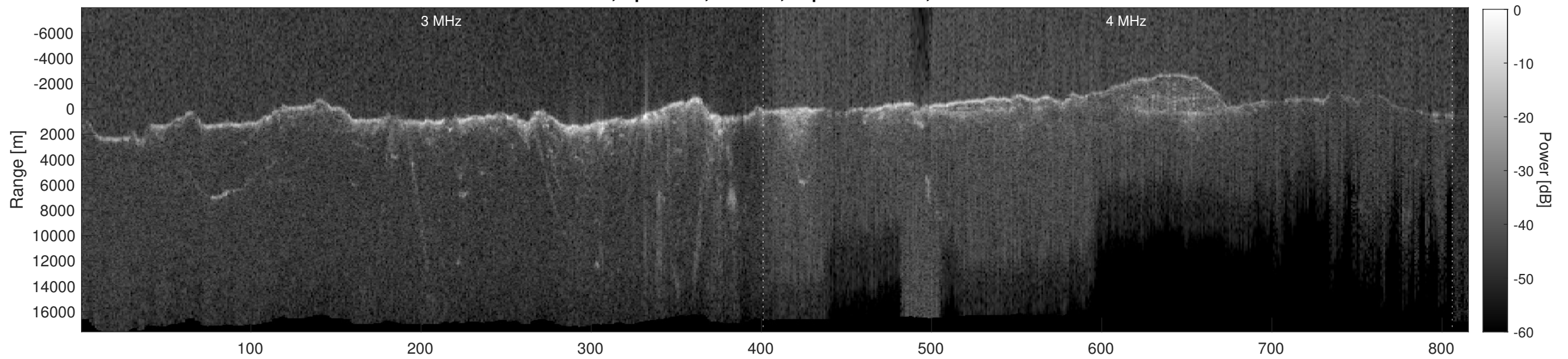
Orbit 6670, Depth-Corrected Cluttergram
