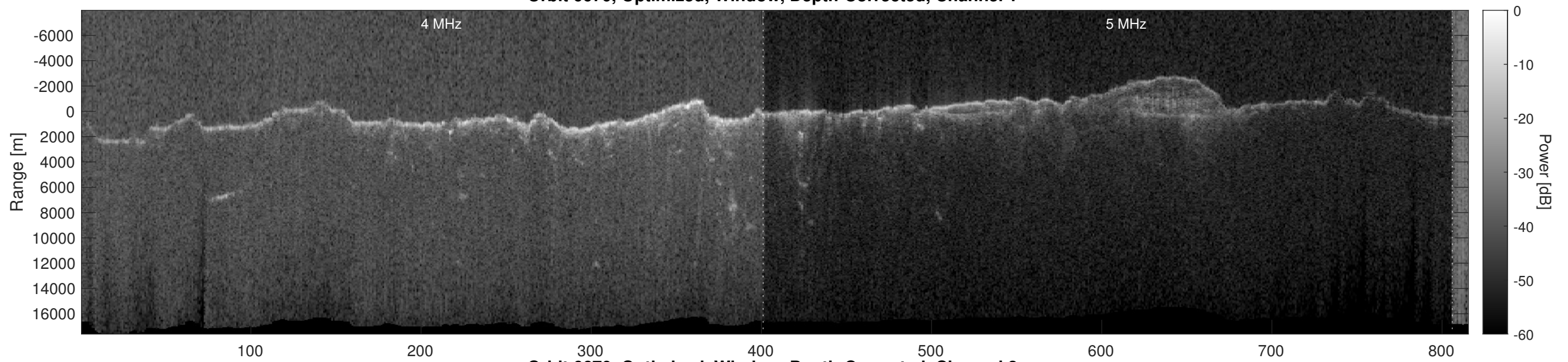
Orbit 6670, Optimized, Window, Depth-Corrected, Channel 2
