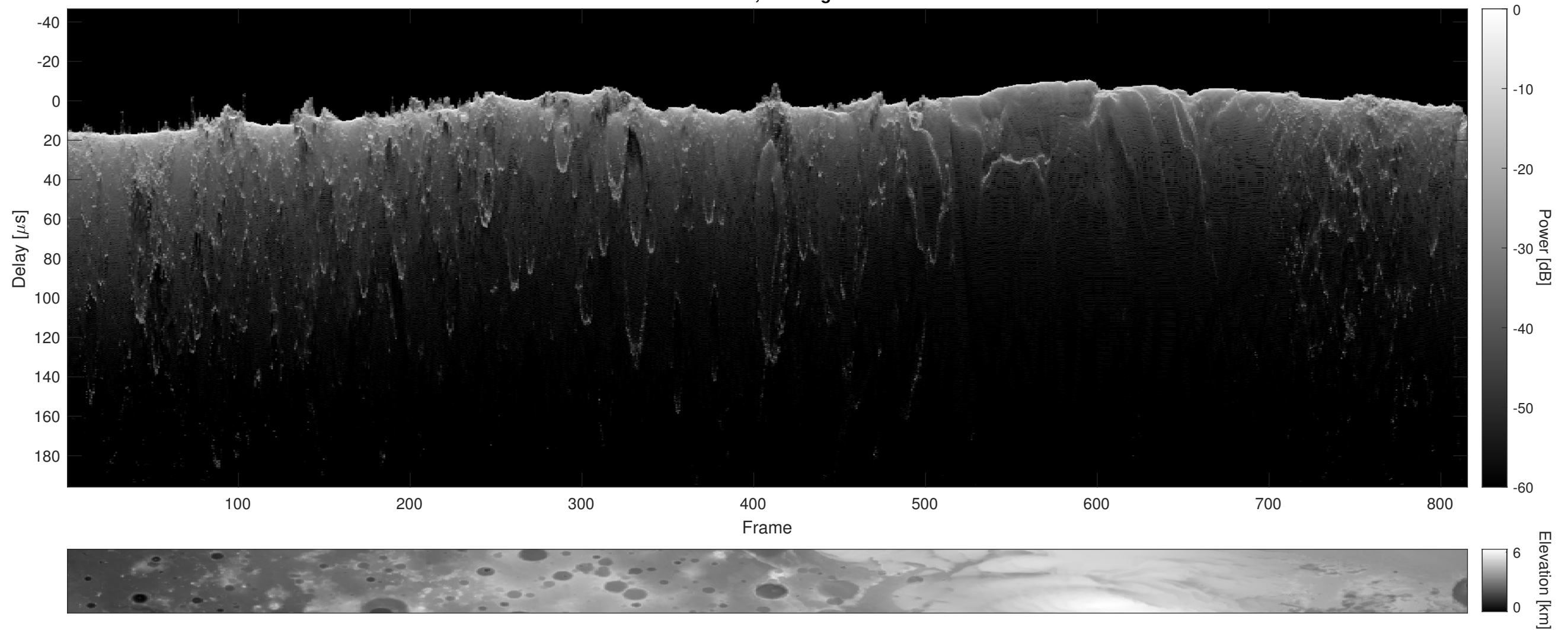
Orbit 6671, Cluttergram
