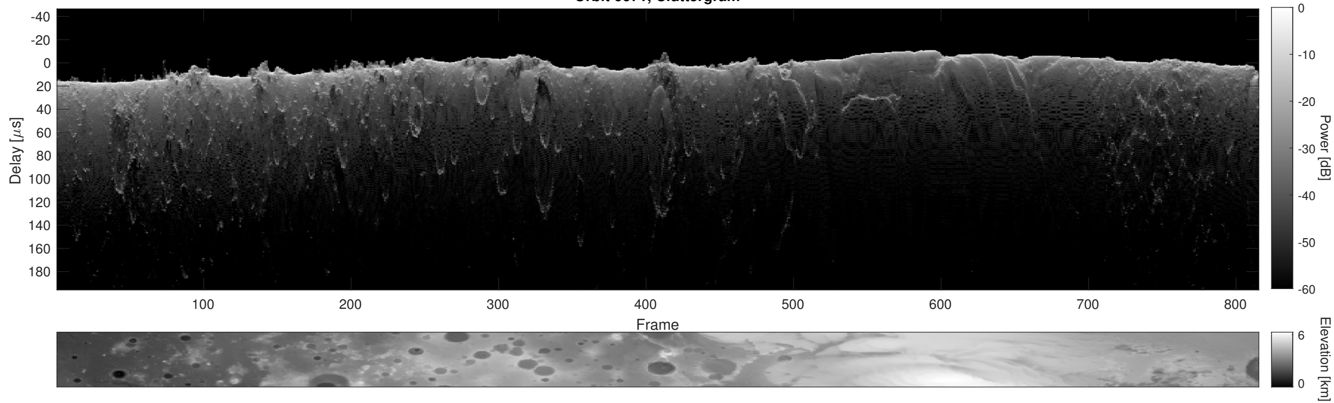
Orbit 6671, Cluttergram
