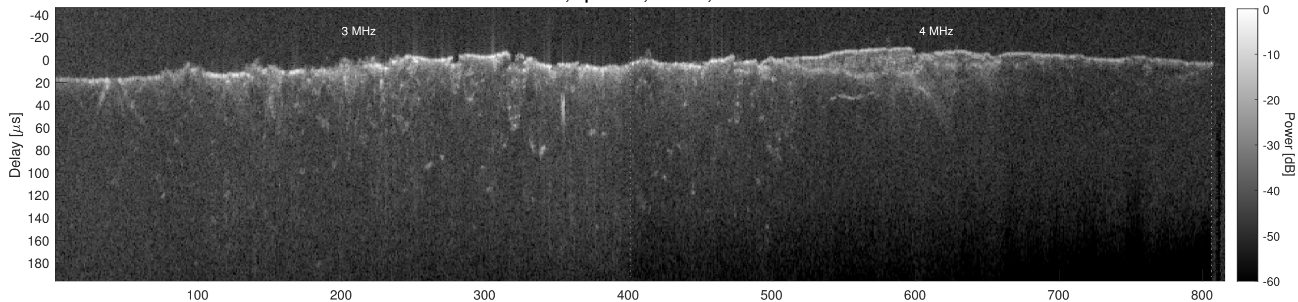
Orbit 6671, Cluttergram
