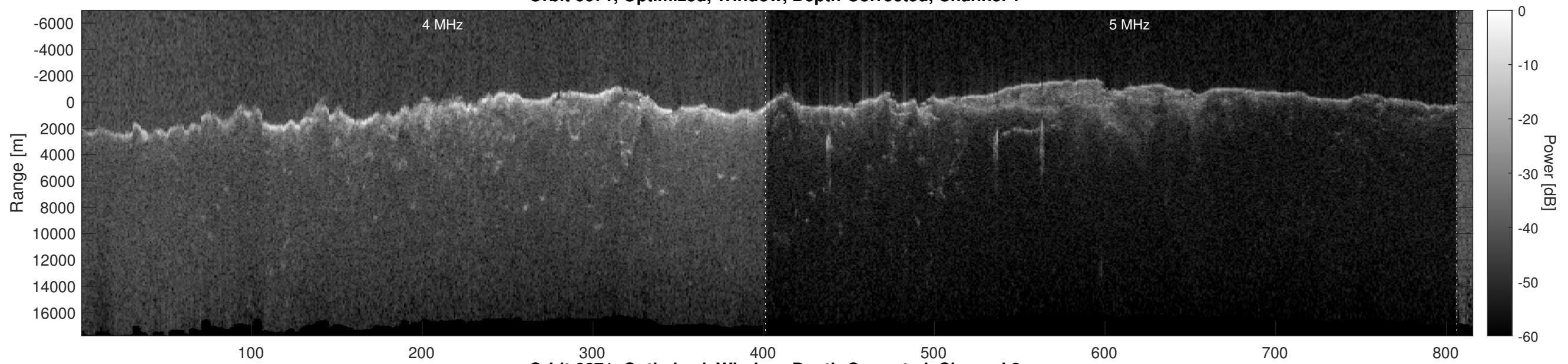
Orbit 6671, Optimized, Window, Depth-Corrected, Channel 2
