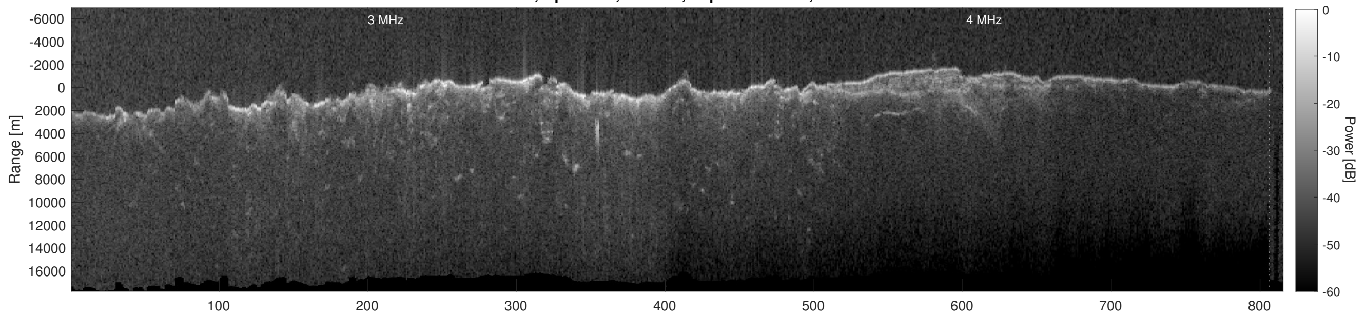
Orbit 6671, Depth-Corrected Cluttergram
