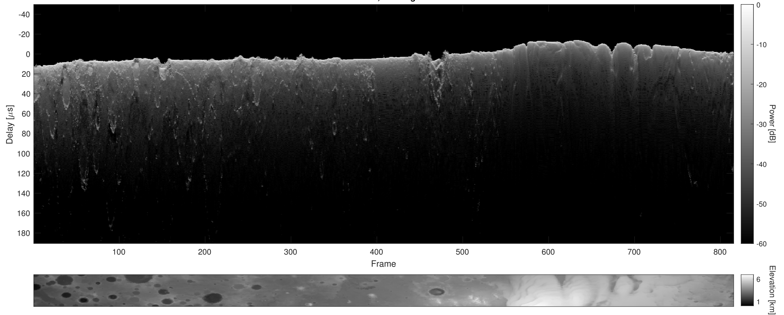
Orbit 6672, Cluttergram
