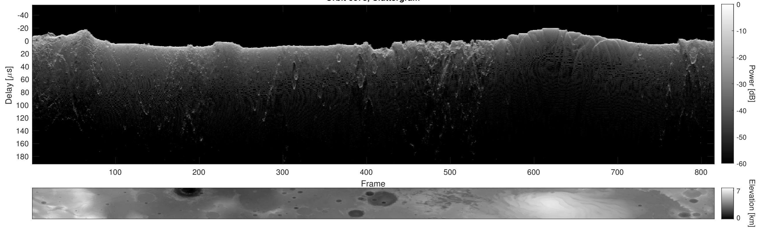
Orbit 6673, Cluttergram
