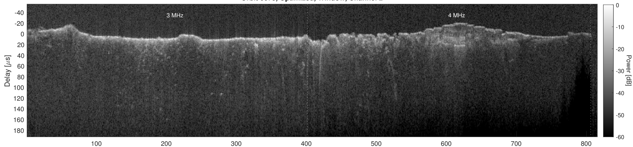
Orbit 6673, Cluttergram
