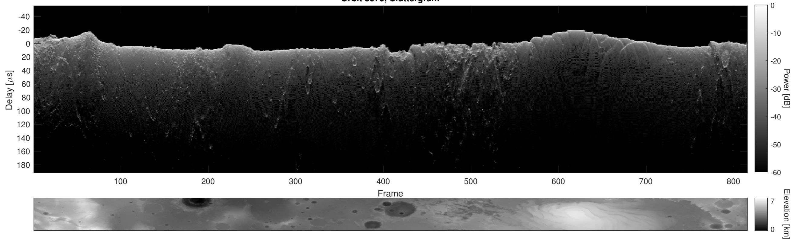
Orbit 6673, Cluttergram
