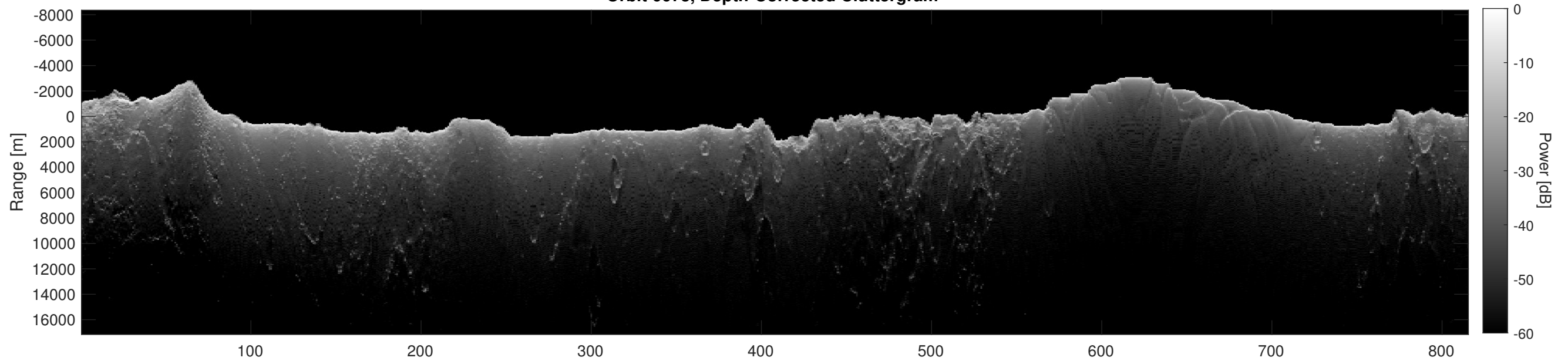
Orbit 6673, Depth-Corrected Cluttergram
