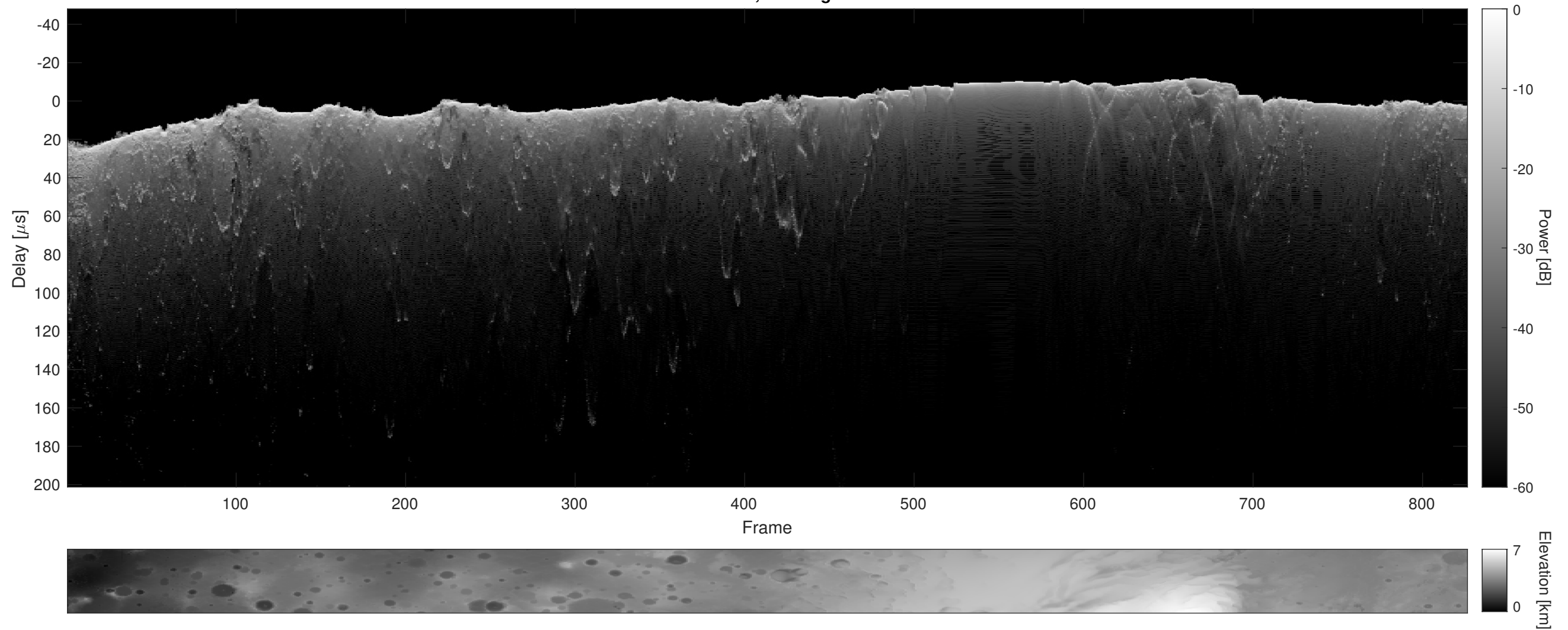
Orbit 6674, Cluttergram
