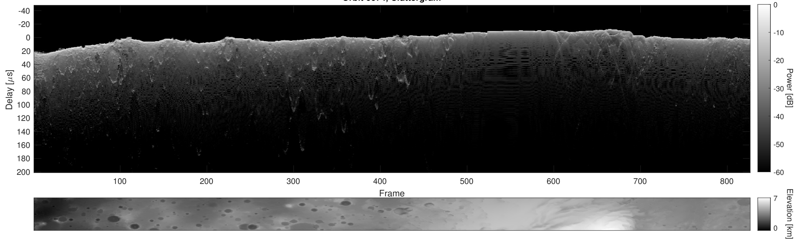
Orbit 6674, Cluttergram
