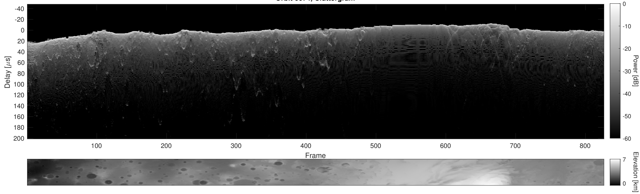
Orbit 6674, Cluttergram
