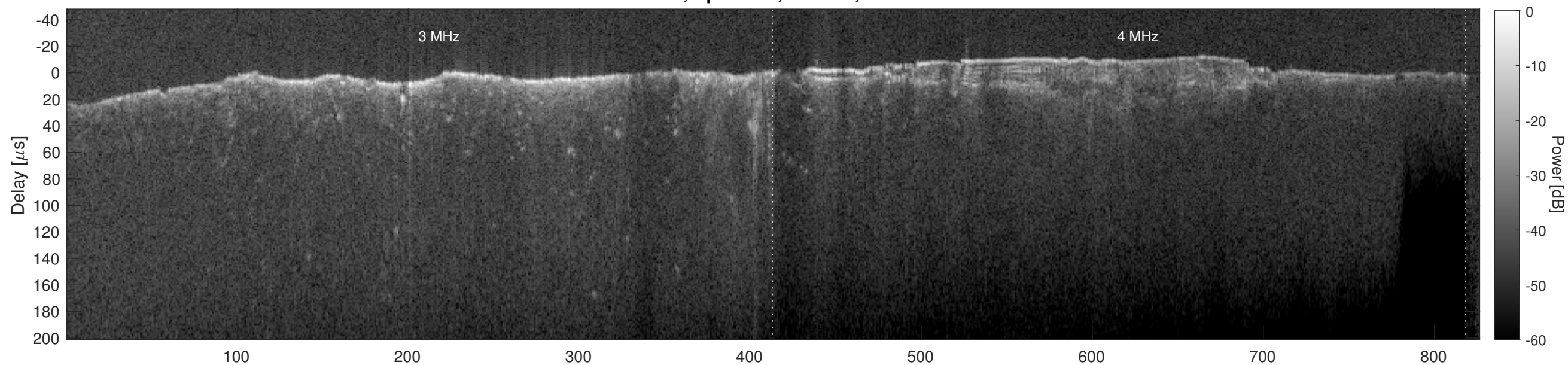
Orbit 6674, Cluttergram
