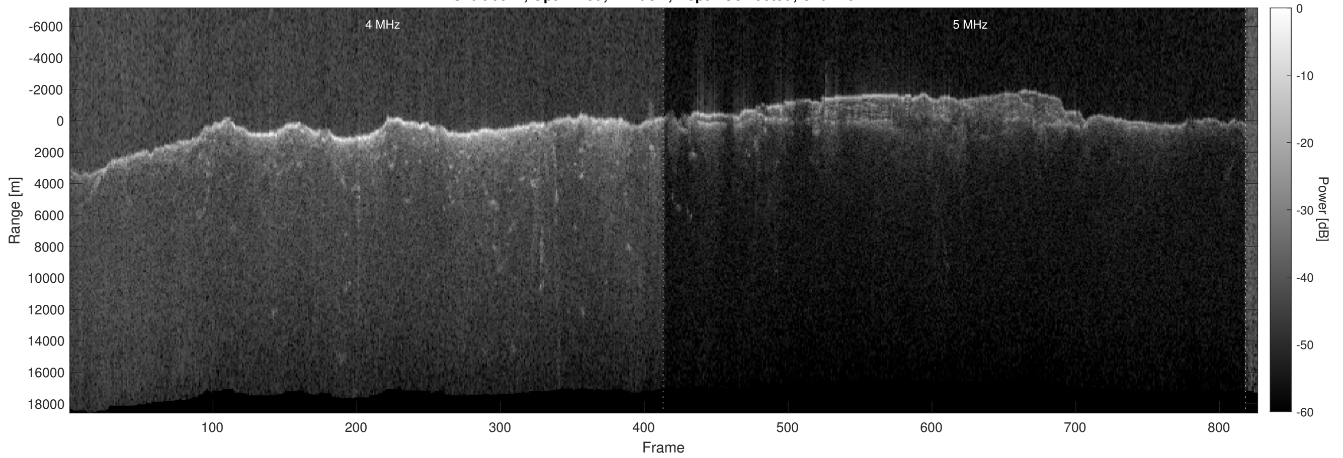
Orbit 6674, Optimized, Window, Depth-Corrected, Channel 2
