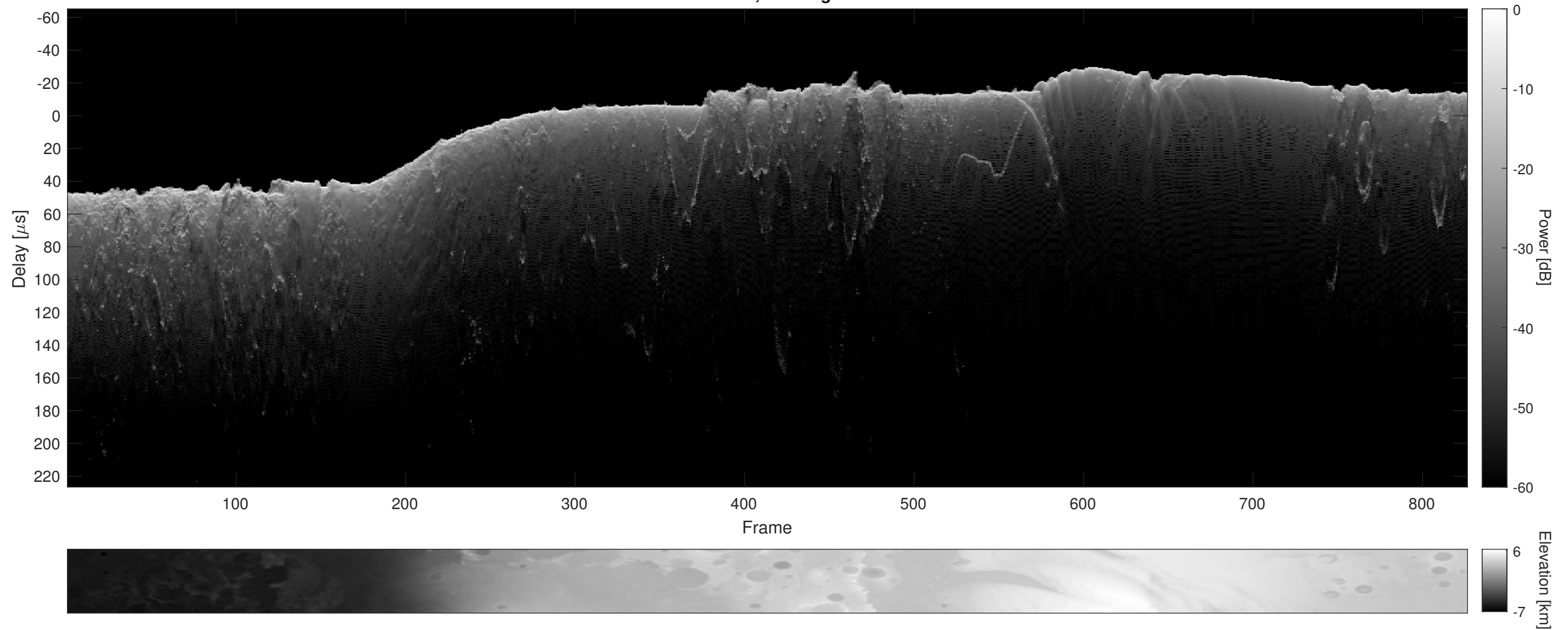
Orbit 6675, Cluttergram
