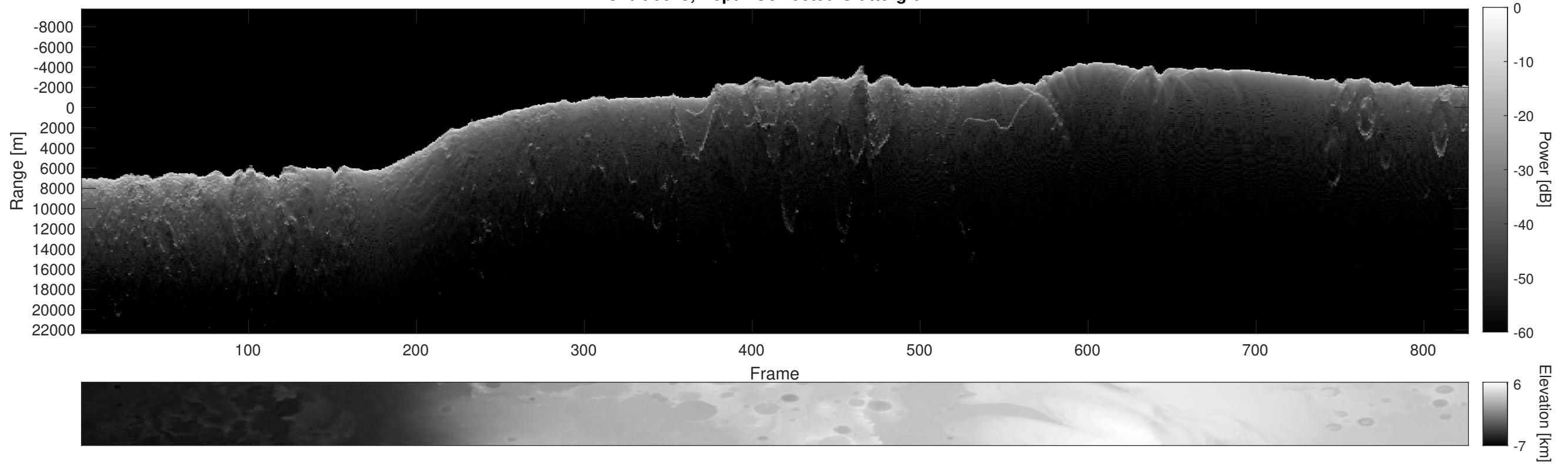
Orbit 6675, Depth-Corrected Cluttergram
