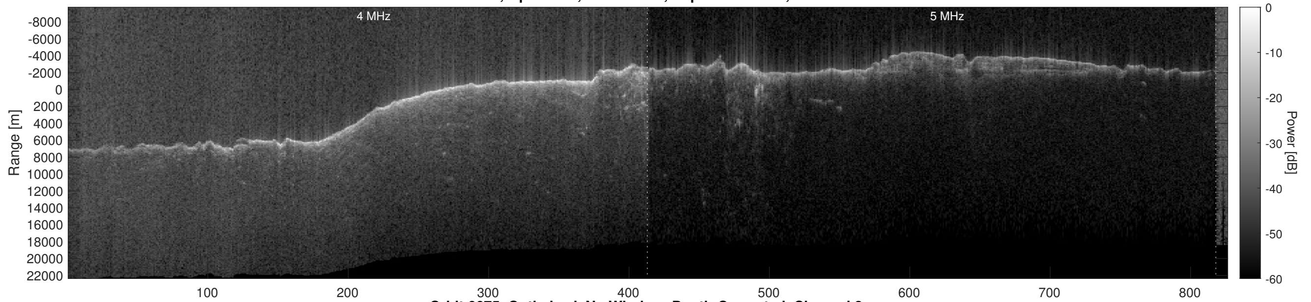
Orbit 6675, Optimized, No Window, Depth-Corrected, Channel 2
