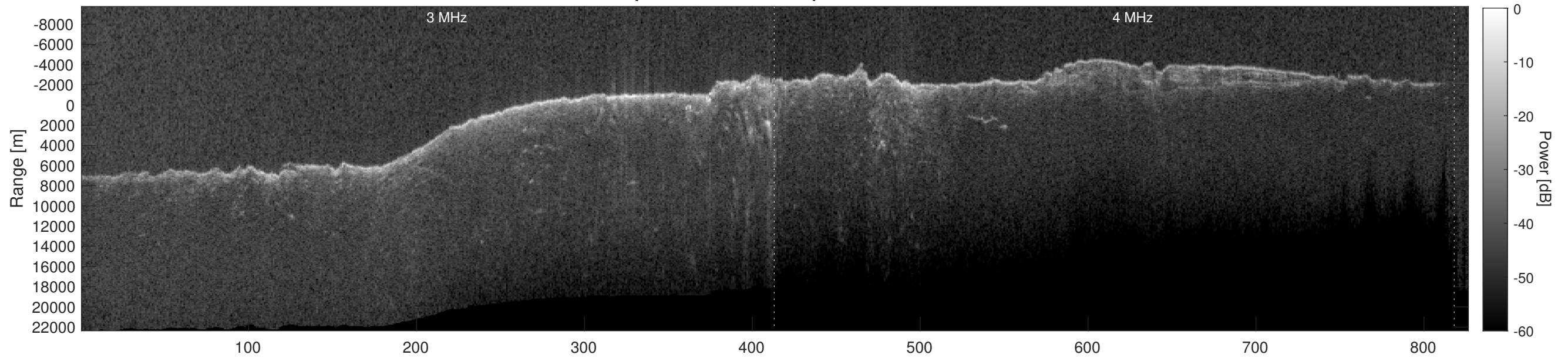
Orbit 6675, Depth-Corrected Cluttergram
