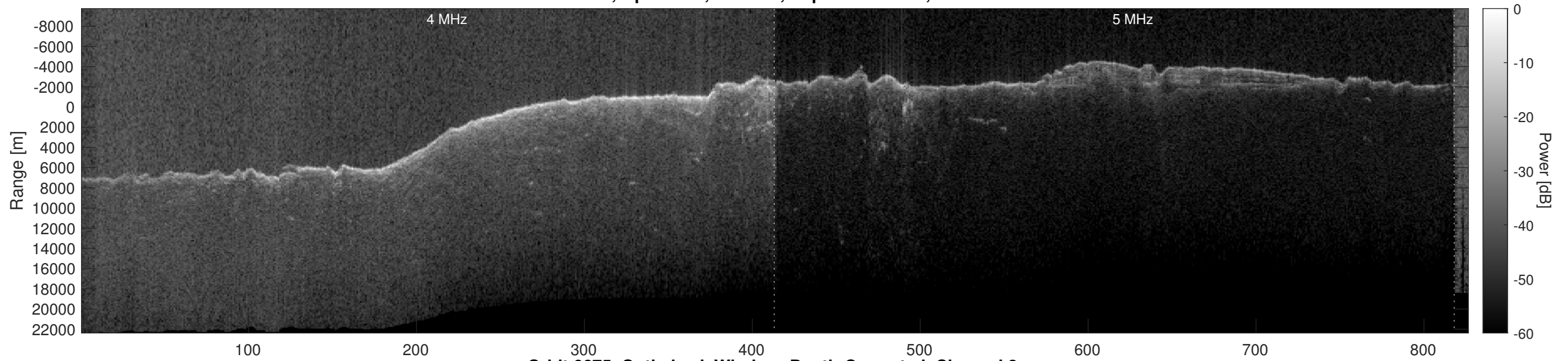
Orbit 6675, Optimized, Window, Depth-Corrected, Channel 2
