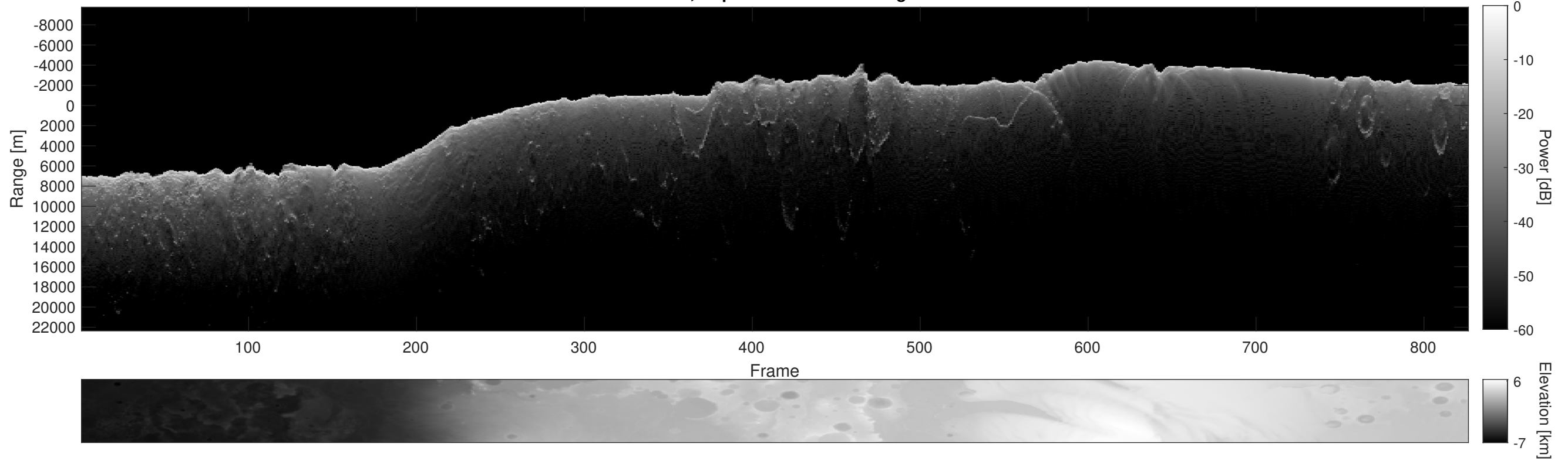
Orbit 6675, Depth-Corrected Cluttergram
