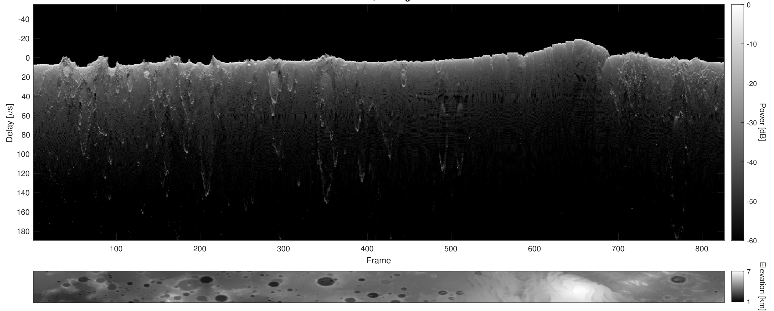
Orbit 6677, Cluttergram
