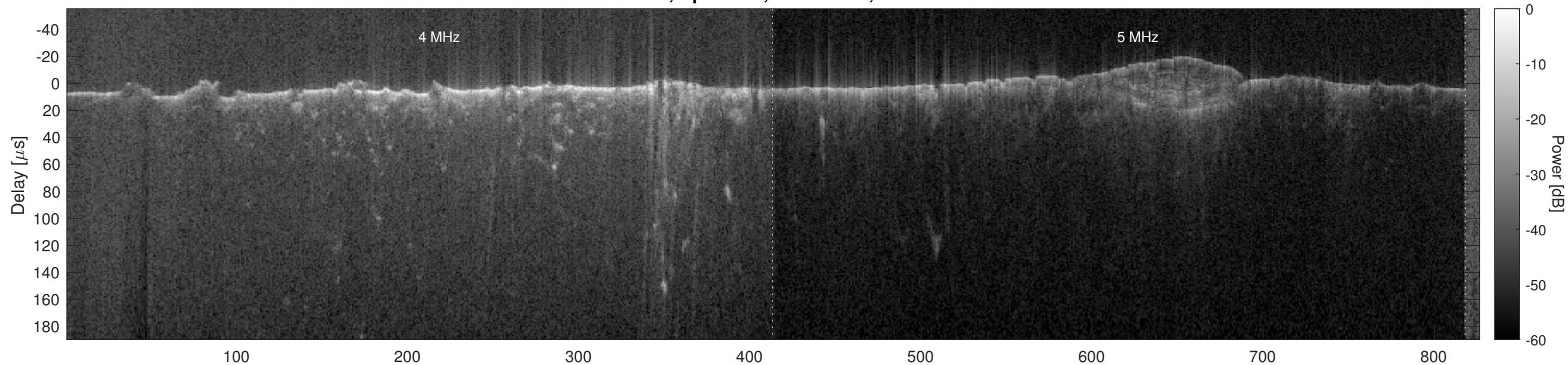
Orbit 6677, Optimized, No Window, Channel 2
