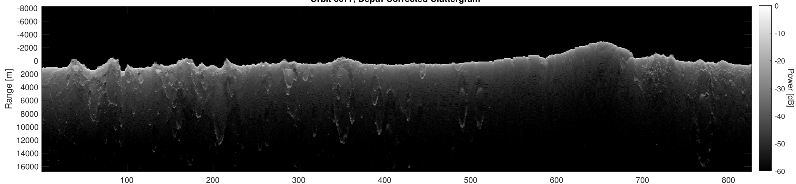
Orbit 6677, Depth-Corrected Cluttergram
