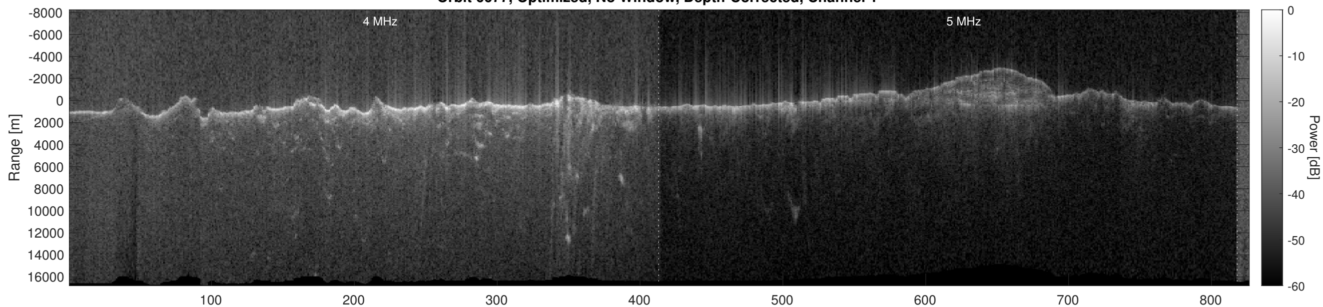
Orbit 6677, Optimized, No Window, Depth-Corrected, Channel 2
