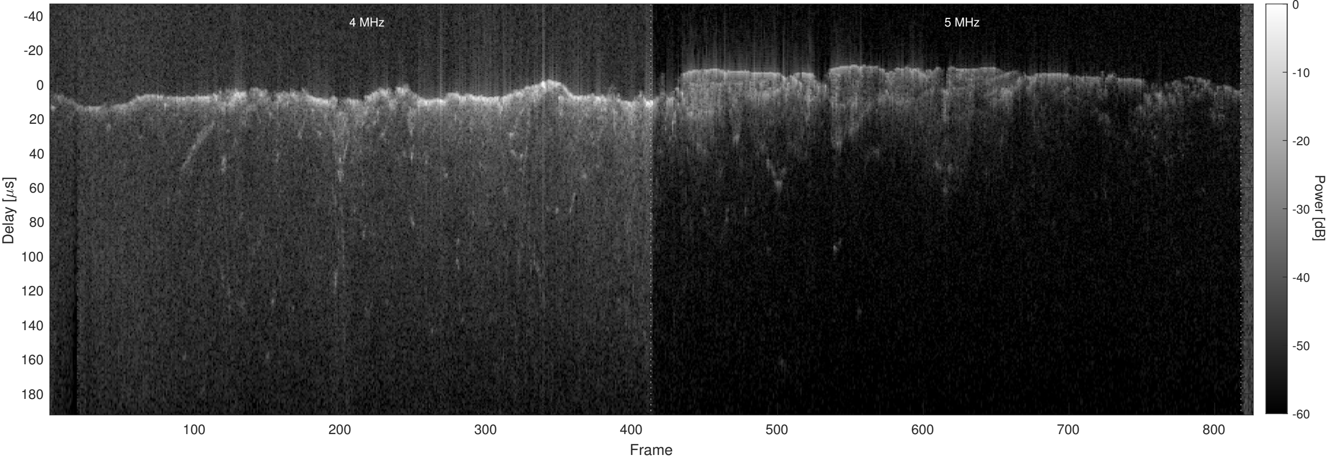
Orbit 6678, Optimized, No Window, Channel 2
