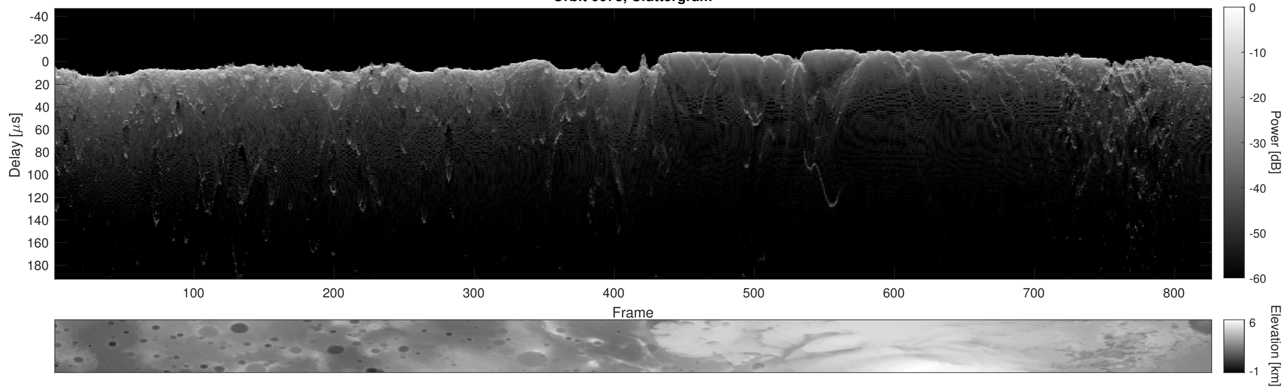
Orbit 6678, Cluttergram
