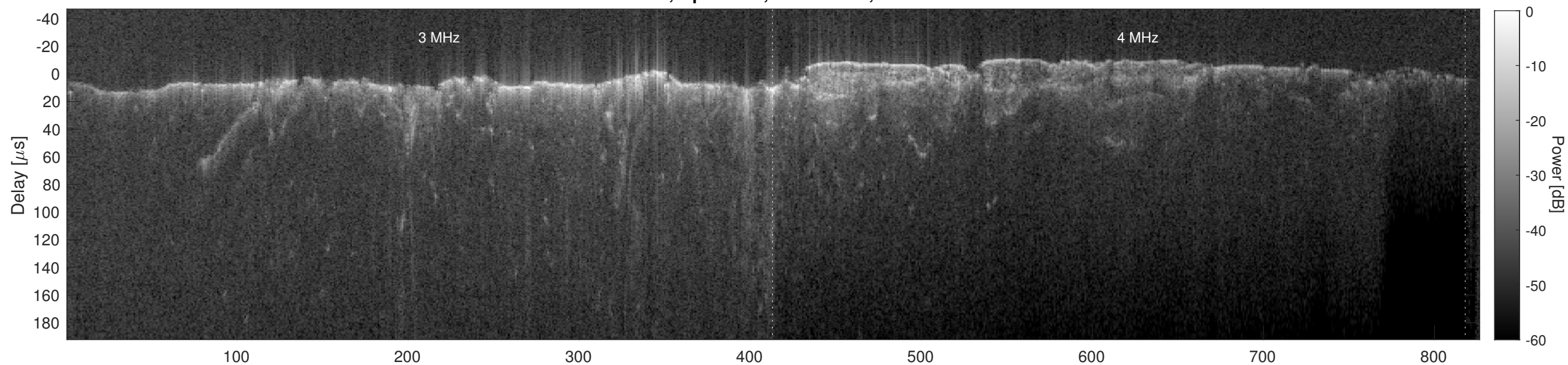
Orbit 6678, Cluttergram
