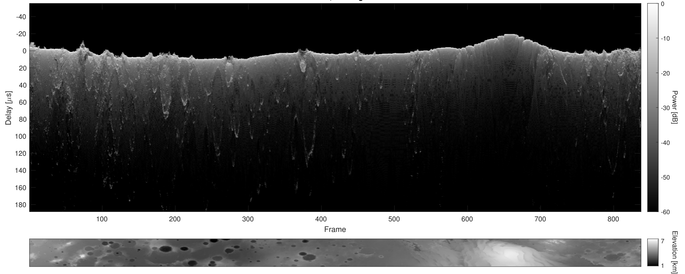
Orbit 6684, Cluttergram
