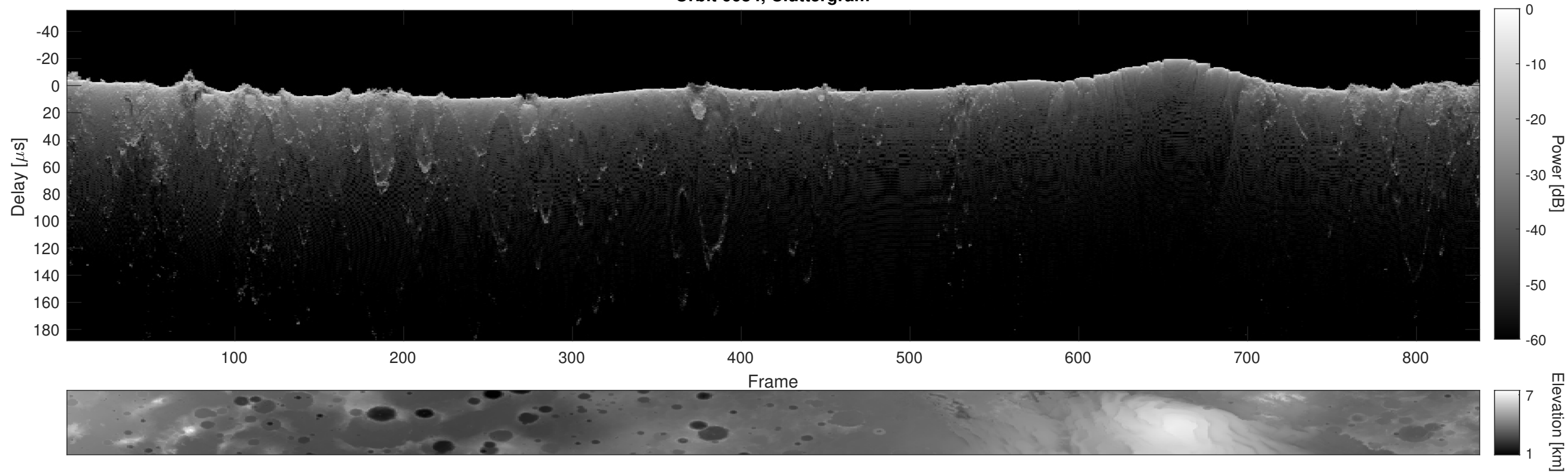
Orbit 6684, Cluttergram
