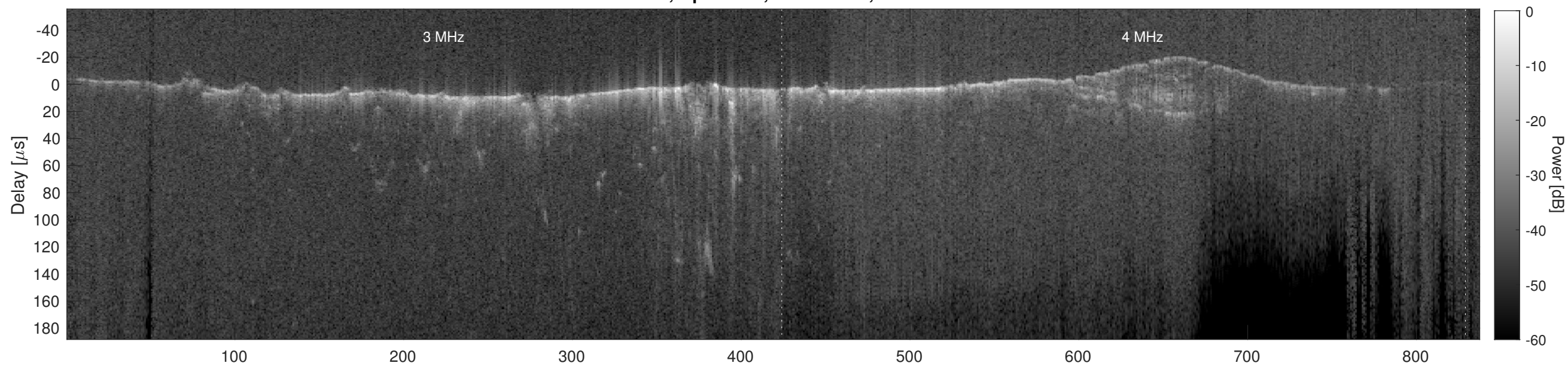
Orbit 6684, Cluttergram
