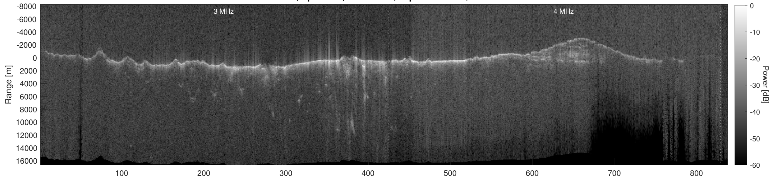
Orbit 6684, Depth-Corrected Cluttergram
