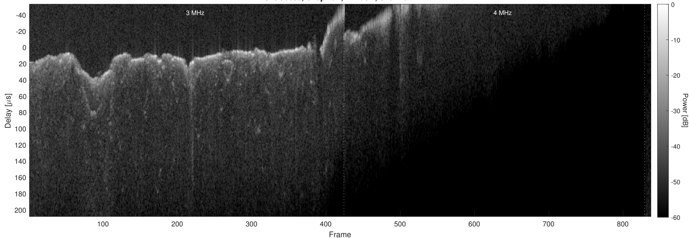
Orbit 6688, Chapman, Window, Channel 2
