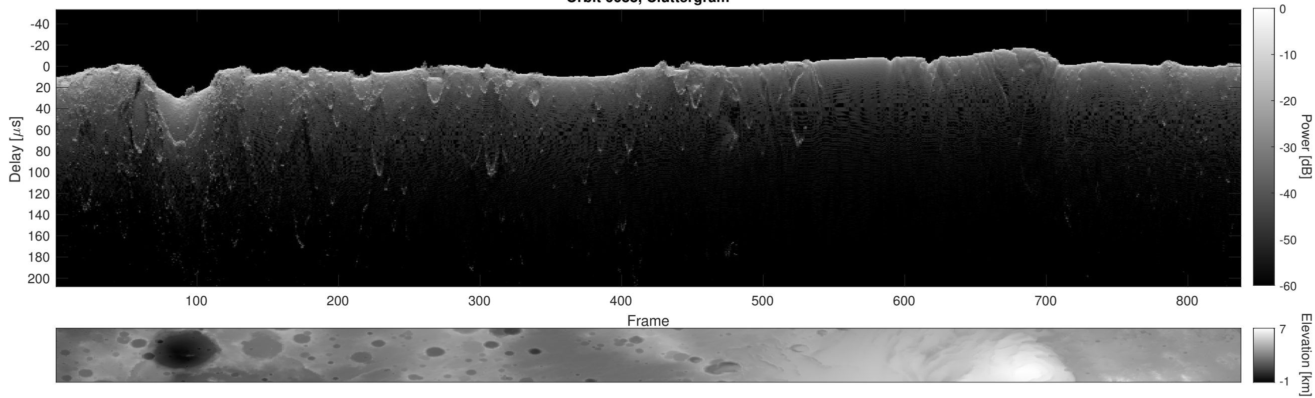
Orbit 6688, Cluttergram
